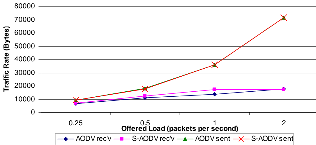
Figure 4.14: Throughput vs Offered Load
